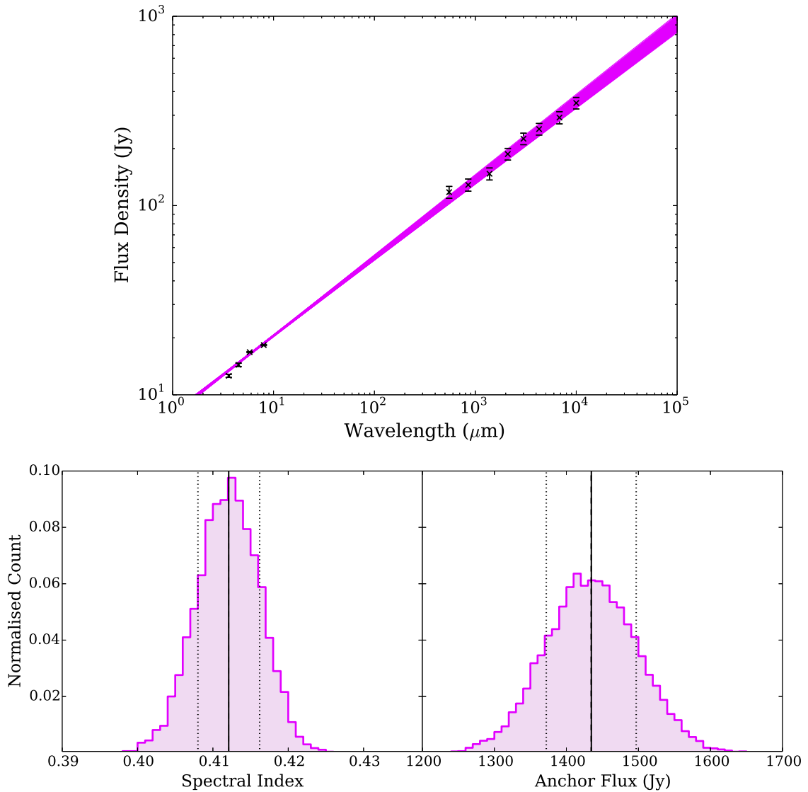
FIGURE 2.14 Upper : Bootstrapped synchrotron spectral energy distribution of the Crab Nebula, showing the 10,000 fits made to randomly perturbed re-samplings of the Spitzer 3.6–8.0 \mu\text{m} and Planck 550–10,000 \mu\text{m} fluxes. Lower : Distribution of parameters generated by performing 10,000 bootstrap fits to the synchrotron SED of the Crab Nebula, using the power law model described by Equation 1.15. Best-fit, bootstrapped median, and bootstrapped confidence intervals are indicated in the same manner as in Figure 2.5. The best fit and bootstrapped median values are in excellent agreement.
