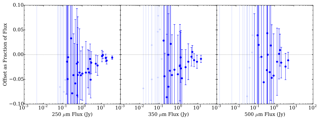
FIGURE 4.7 Source flux versus offset due to sky annuli as a fraction of source flux, as described in Equation 4.2, for the HAPLESS sources in all three SPIRE bands. Full-colour data points are > 5\sigma detections, whilst faint data points are not.
