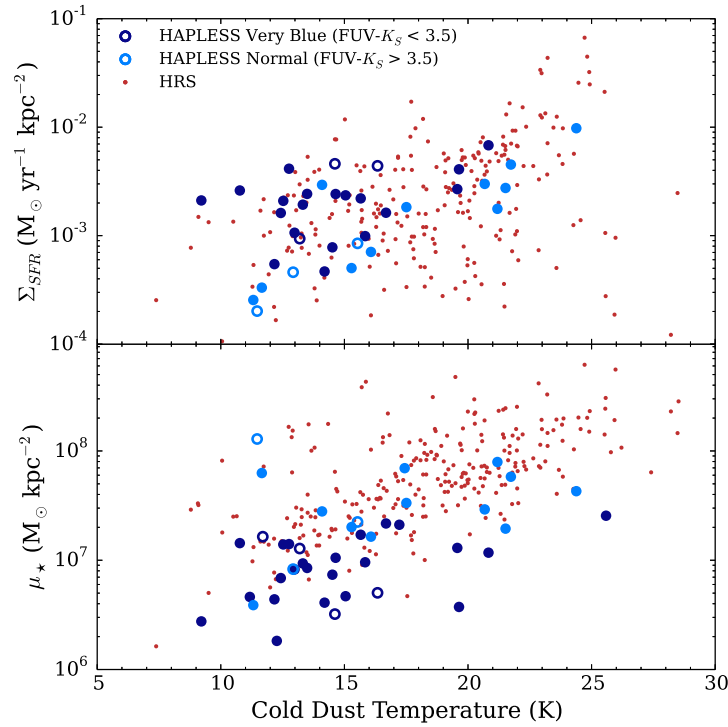
FIGURE 6.14 The variation of SFR surface density, \Sigma_{SFR} , ( upper ), and the stellar mass surface density, \mu_* , ( lower ), with cold dust temperature for the HAPLESS and HRS galaxies.
