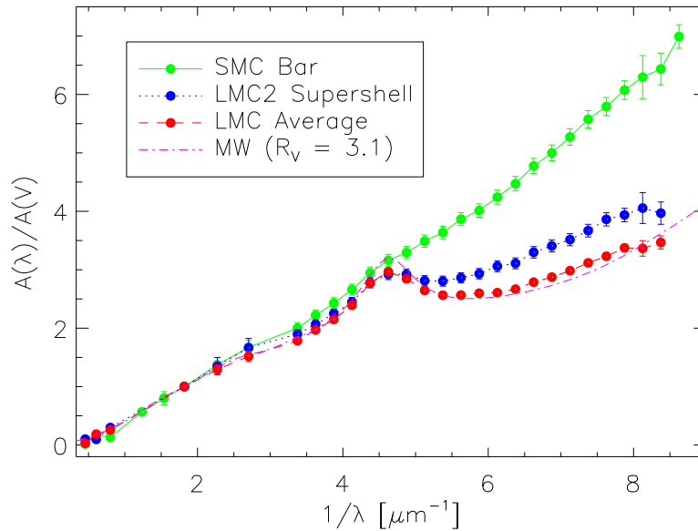
FIGURE 1.4 Extinction curves of the Milky Way and Magellanic Clouds. The term R_V , stated to be 3.1 for the Milky Way, is defined by R_V = A_V/E(B - V) (ie, gives extinction in V -band, relative to the B - V reddening). Reproduced from Gordon et al. (2003) , under the Creative Commons Attribution-ShareAlike 3.0 Unported license.
