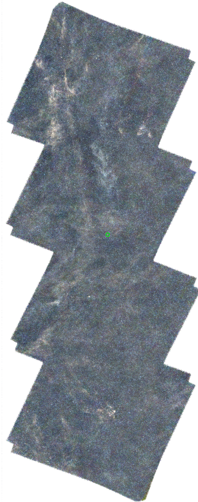
FIGURE 3.5 Three-colour SPIRE (250, 250, and 500 \mu\text{m} ) images of the H-ATLAS GAMA fields, with the locations of the HAPLESS galaxies indicated by the green circles. This Page: The H-ATLAS GAMA09 field.
