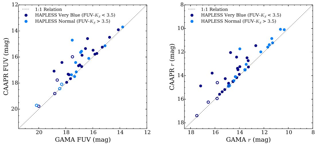
FIGURE 4.5 Comparison of photometry of the HAPLESS galaxies provided by the GAMA pipeline of Hill et al. (2011), to the photometry produced by CAAPR, in the FUV (left) and r -band (right). Note the large fraction of galaxies for which CAAPR returns significantly brighter magnitudes; this is particularly prone to happening in the case of the very blue HAPLESS galaxies. Whether a point is blue or cyan denotes the FUV-K_S colour of the source, as separated by the FUV-K_S = 3.5 criterion, with hollow circles indicating galaxies not in the luminosity-limited sub-sample.
