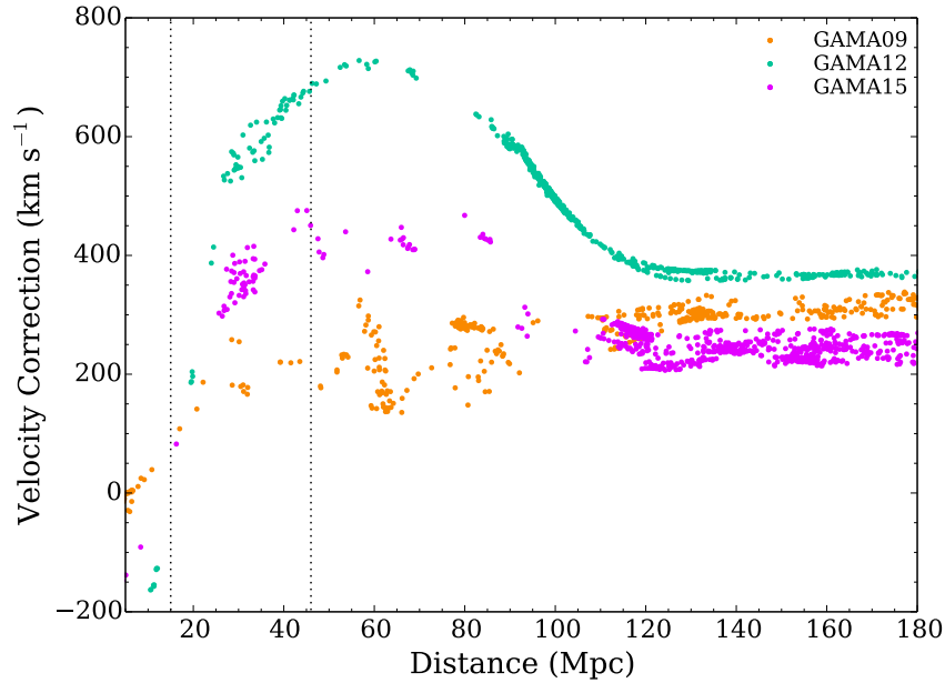
FIGURE 3.2 The velocity correction applied to each source in the GAMA fields out to D = 180 Mpc, determined according to the method of (Tonry et al., 2000), which accounts for the motion of the Local Group relative to the CMB due to the gravitational influence of the Virgo Cluster and the Great Attractor. The particularly pronounced velocity corrections required in the GAMA12 field are due to its proximity to the Virgo Cluster. The dotted lines indicate the 15 and 46 Mpc distance limits of the HAPLESS sample.
