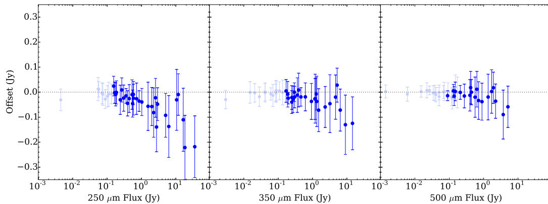
FIGURE 4.6 Source flux versus offset due to sky annuli, as described in Equation 4.1, for the HAPLESS sources in all three SPIRE bands. Full-colour data points are > 5\sigma detections, whilst faint data points are not.
